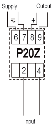
Fig.1 Direct measurement of voltage
